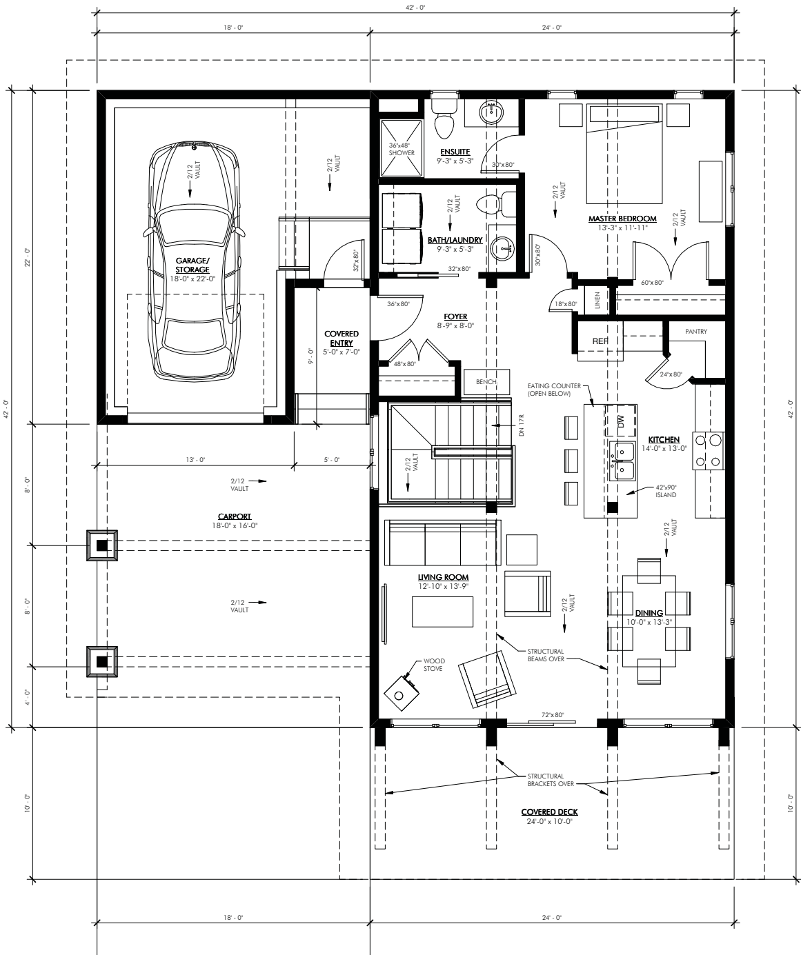
MAIN FLOOR PLAN AREA: 1008 SQ FT 1/4" = 1'-0"
